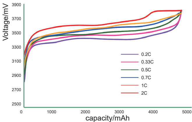
Charging curve
