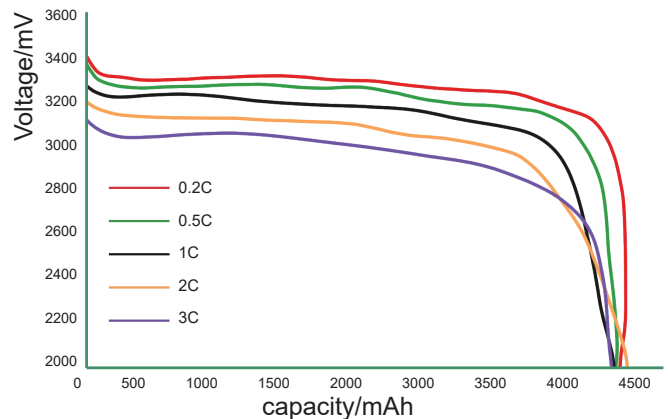
Discharge curve
